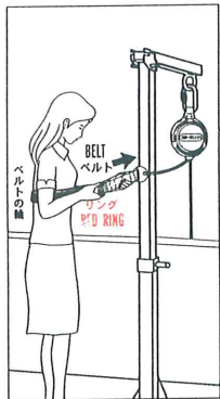
FASTEN THE BELT WITH RED RING IN YOUR FRONT POSITION. AND TIGHT THE BELT.
